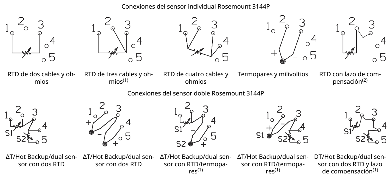
Figura 8: HART®/4–20 mA
