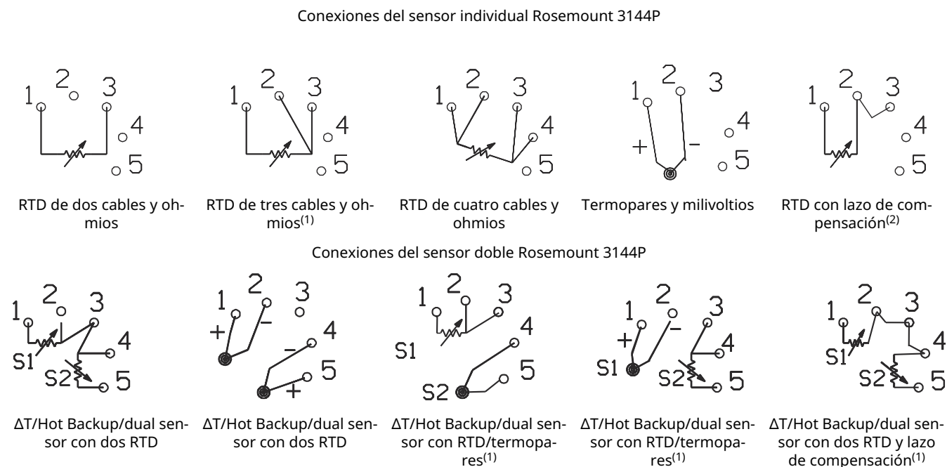
Figura 9: FOUNDATION Fieldbus
